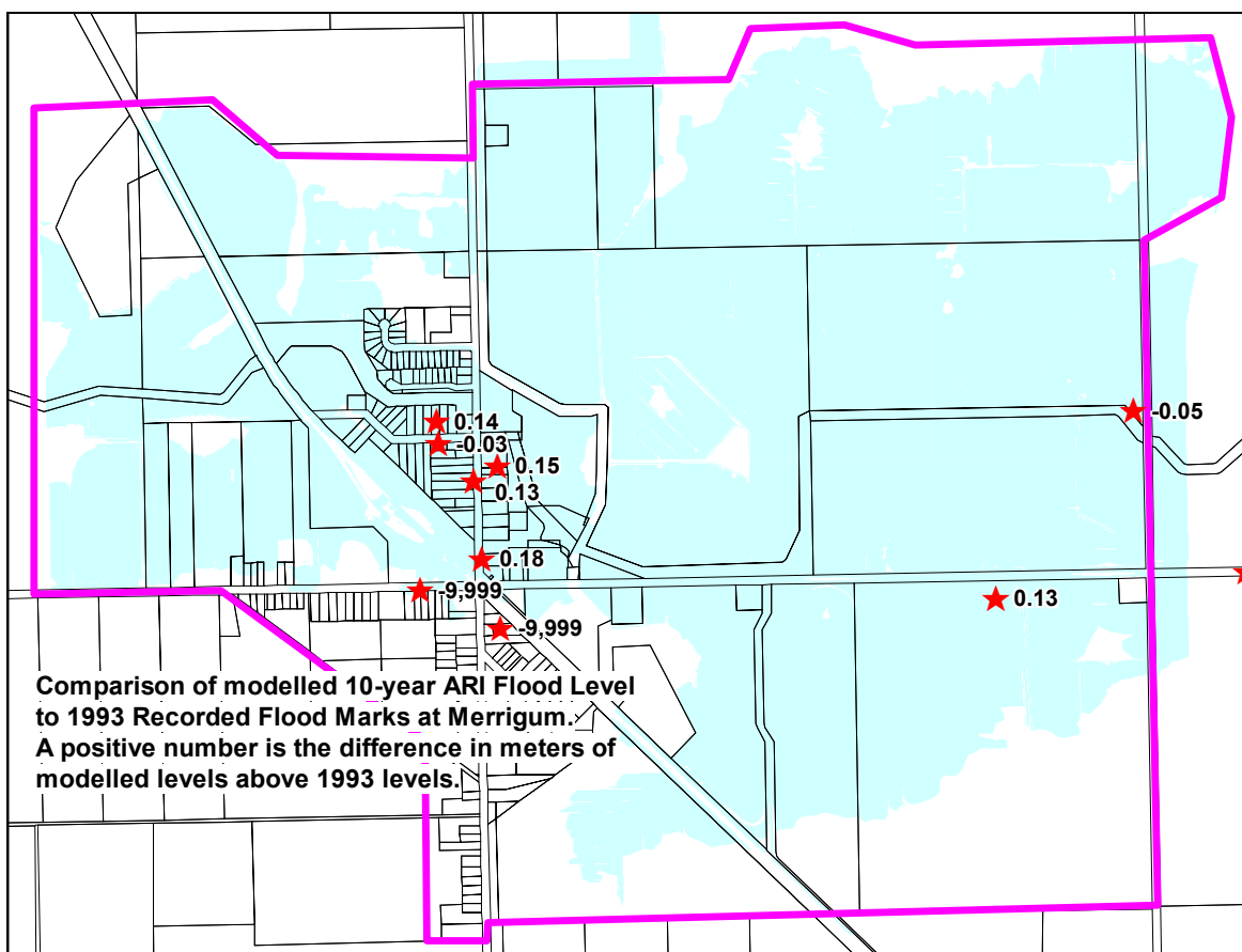
Figure 5-1 Comparison of Modelled 10-year ARI Peak Flood Levels and October 1993 Flood Marks*
