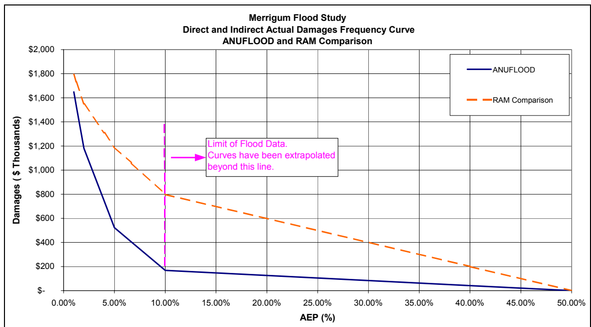
Figure 6-4 ANUFLOOD Damages Curve
