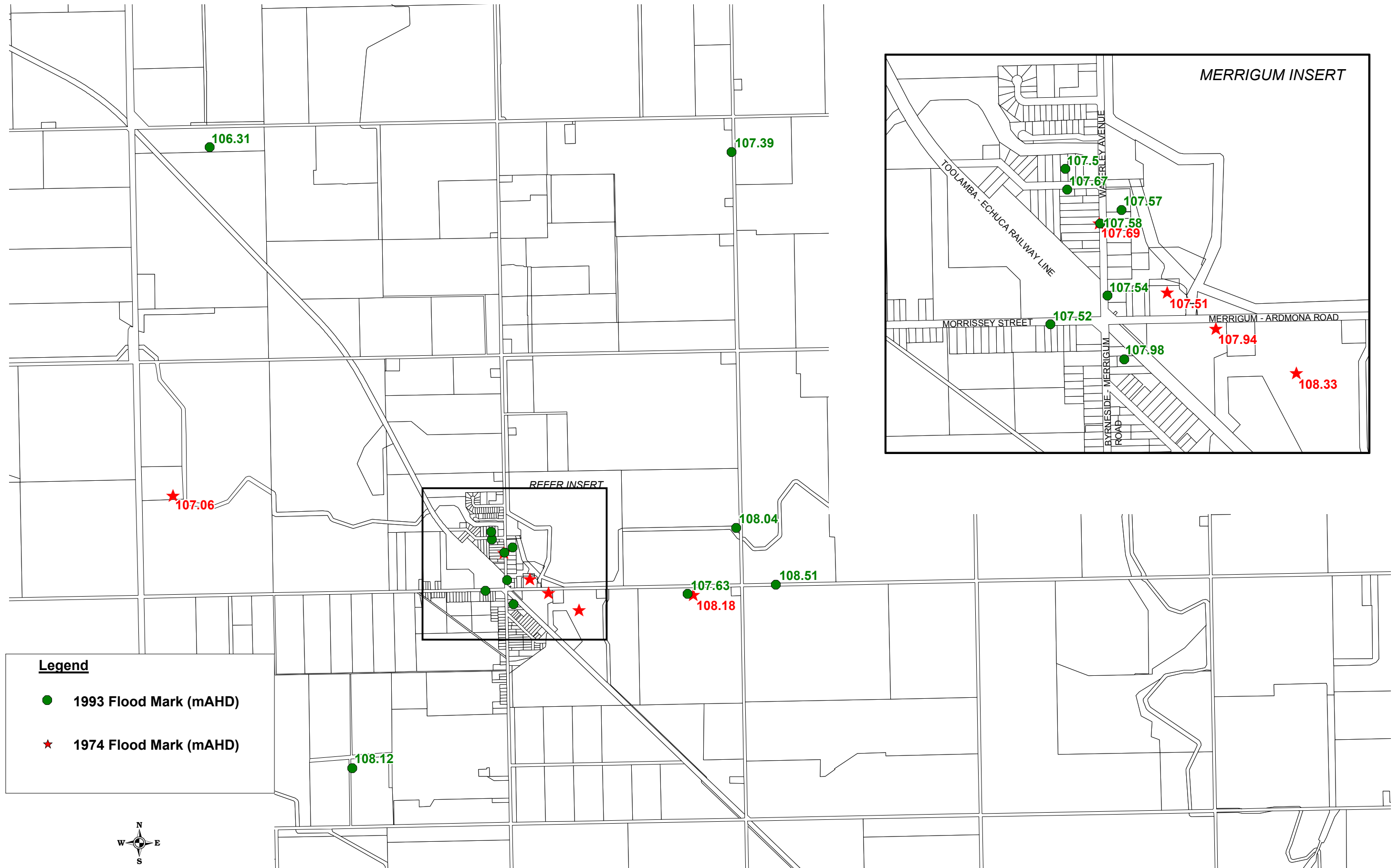
Distribution of Historical Flood Marks for the Mosquito Depression at Merrigum
