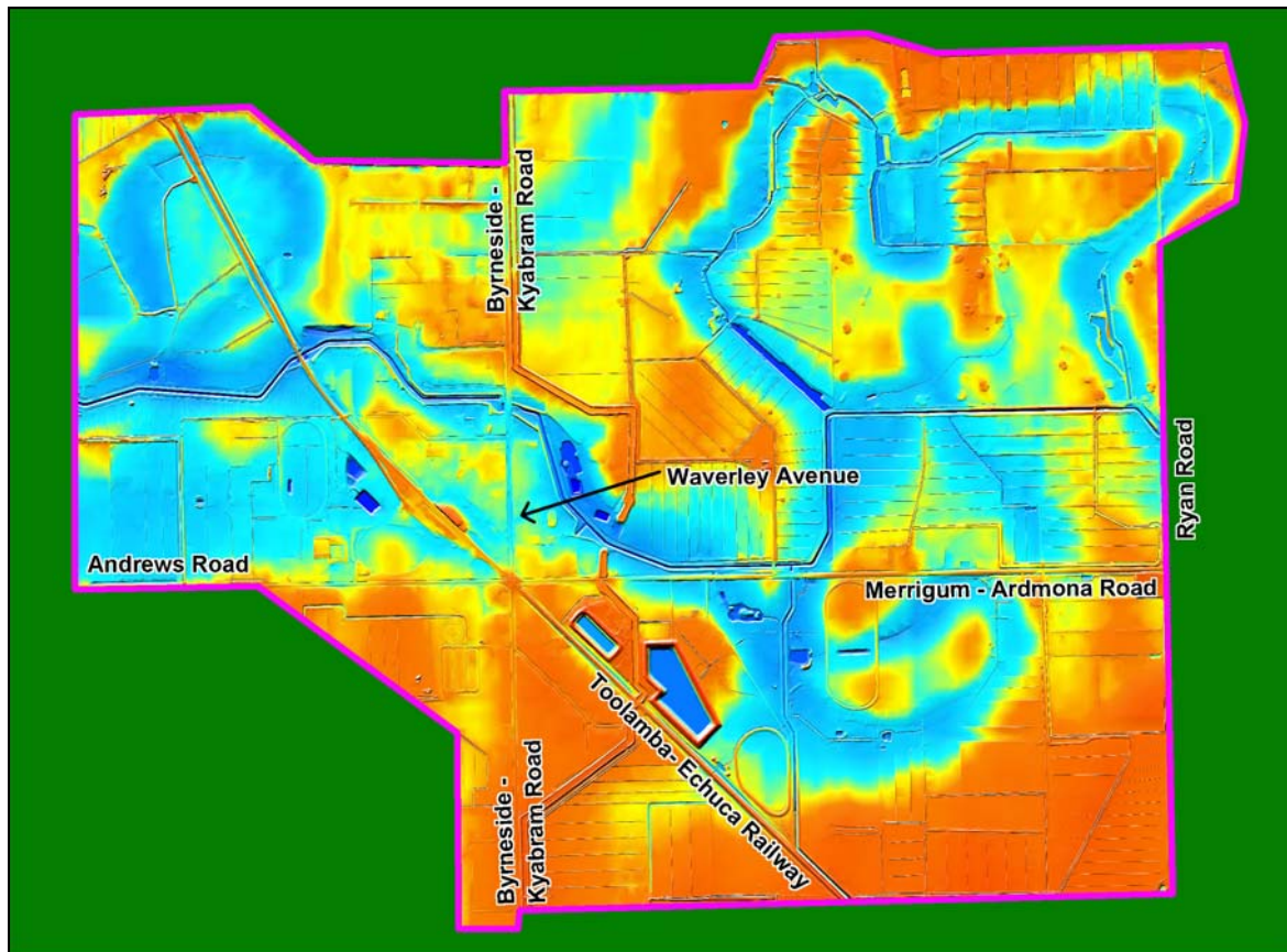
Figure 2-1 Merrigum Study Area DEM
